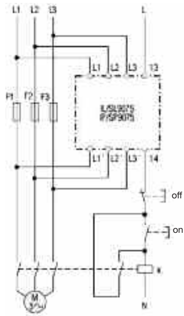
Fuse-monitoring in 3-phase-network
