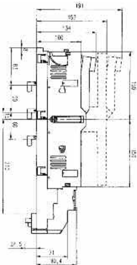
Size 00, Order no.: 38534-1000
